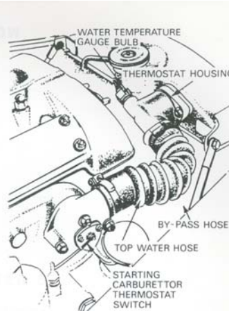
FIG 4:6 Thermostat, XK120 model
