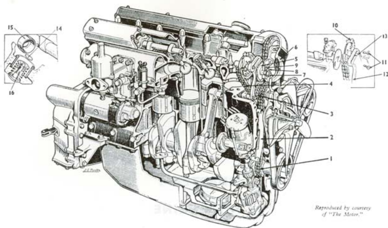
FIG 1:1 The Jaguar XK engine
