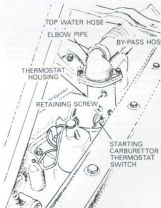
FIG 4:7 Thermostat, Mk VII model
